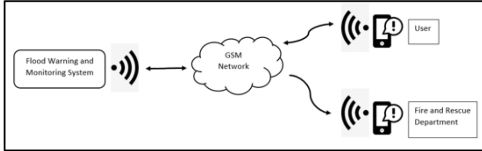
Figure 2: Proposed architecture
